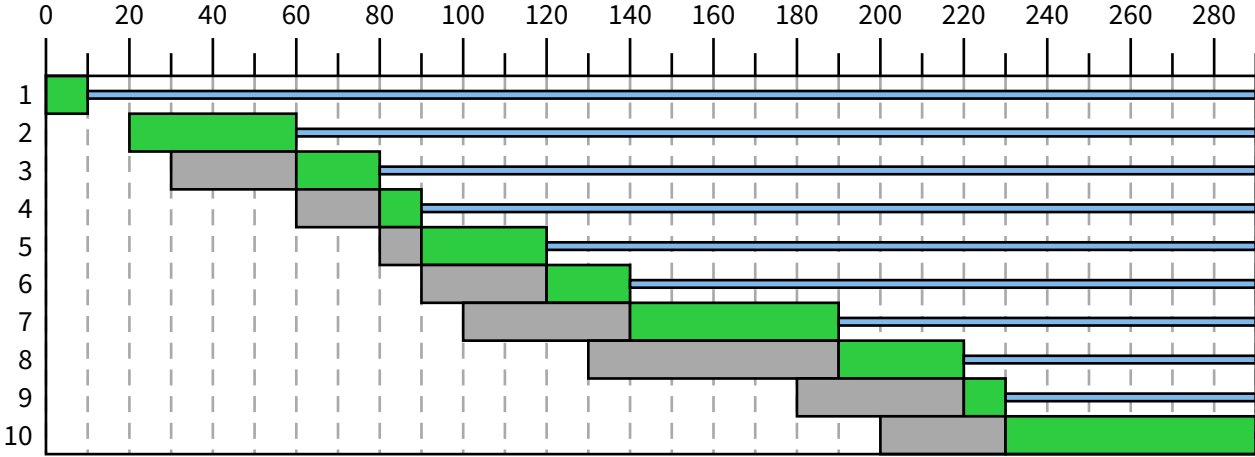
Figure 1: Process scheduling: FCFS
