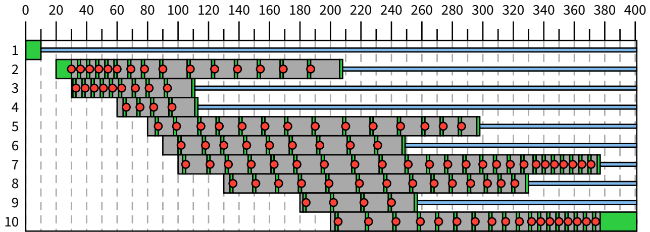
Figure 4: Process scheduling: RR
