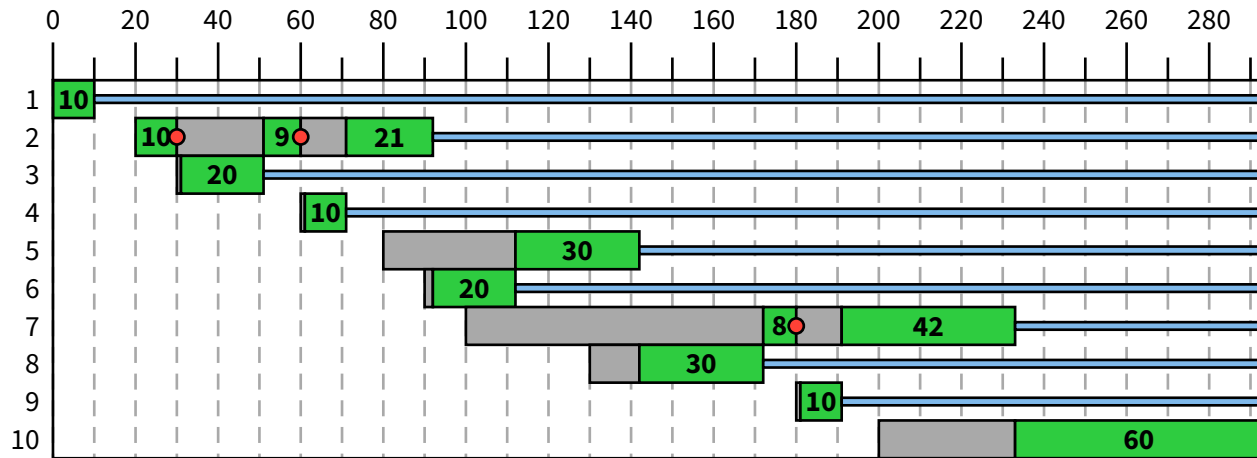
Figure 3: Process scheduling: SRTF
