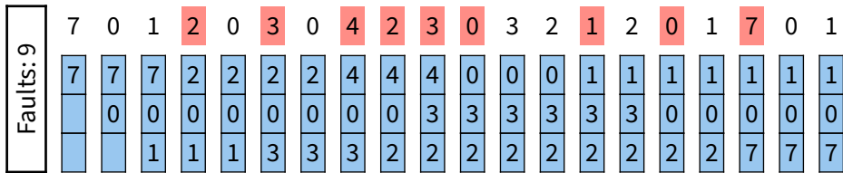
Figure 3: Demand Paging: LRU
