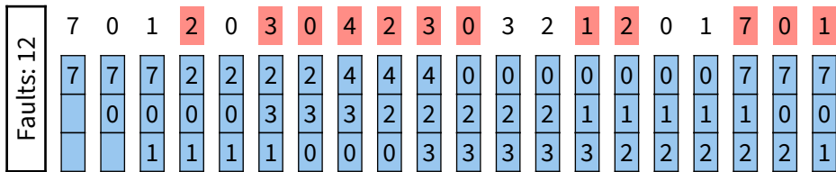
Figure 1: Demand Paging: FIFO
