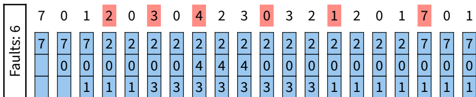
Figure 2: Demand Paging: OPT
